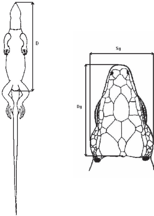
Fig. 1. The main traits in lizards (after MAJLÁTH et al. 1997 – modified): body length (D), head length (Dg), head width (Sg).
