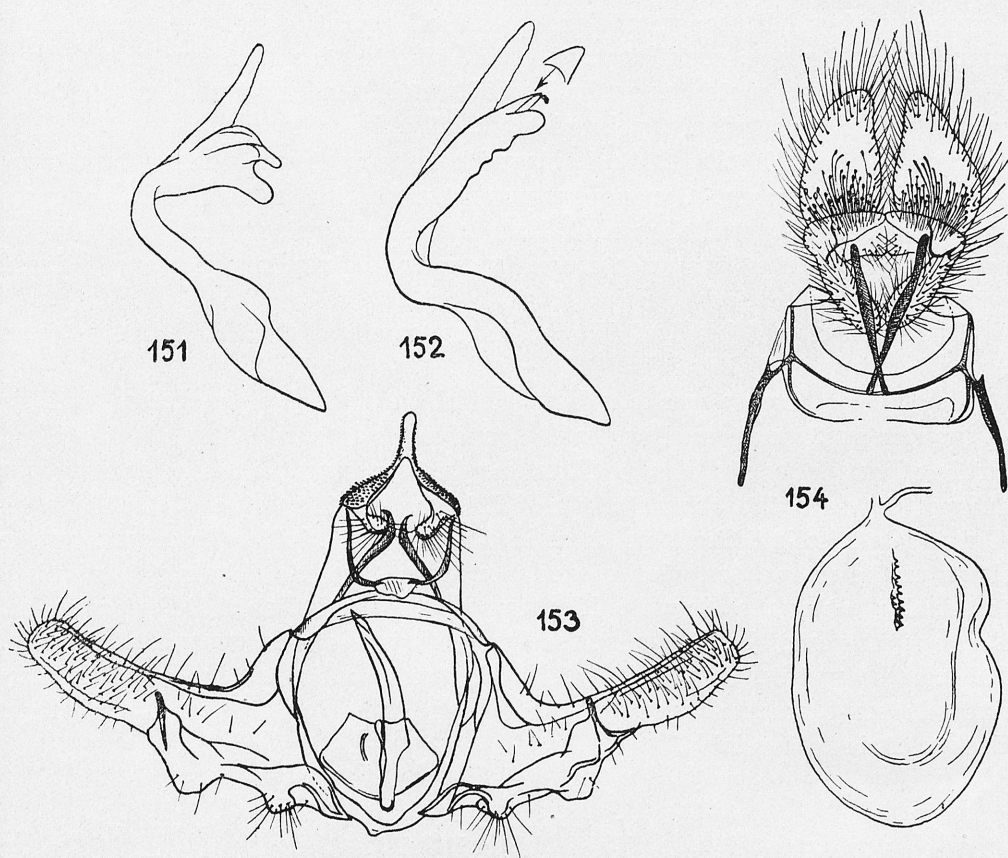
Figs. 151—154. Male and female genitalia: 151 — valva of Doloploca praeviella (ERSCH.) ventrally, 152 — valva of D. buratica STGR., ventrally, 153 — D. characterana SNELL., „Sutshan, 95, leg. DÖRR, ex. coll. STGR.“, G. Sl. 3273 (Berl.), 154 — same species, female, „Ush. Sutsuktie, in.-z. Kiutiei, Mongolia, 12. VI. 924, KOZLOV“, G. Sl. 4918
