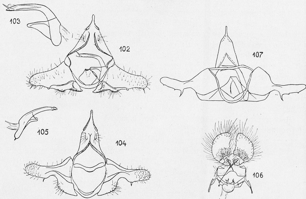
Figs. 102—107. Male and female genitalia: 102 — Oxypteron algerianum sp. n., otype, 103 — aedeagus of same specimen, 104 — O. eremicum (WALSM.), type, „Hamnan-es-Salahin, Algeria, 15. III. 1904“, G. Sl. 5677 (BM), 105 — aedeagus of same specimen, 106 — same sp., female, „Gafsa, 18. XI. [19]08, Type [of O. partitanum CHRÉT.]“, G. Sl. 3726 (VIETTE), 107 — O. homsanum AMS., holotype (reconstr. after AMSEL, 1954)
